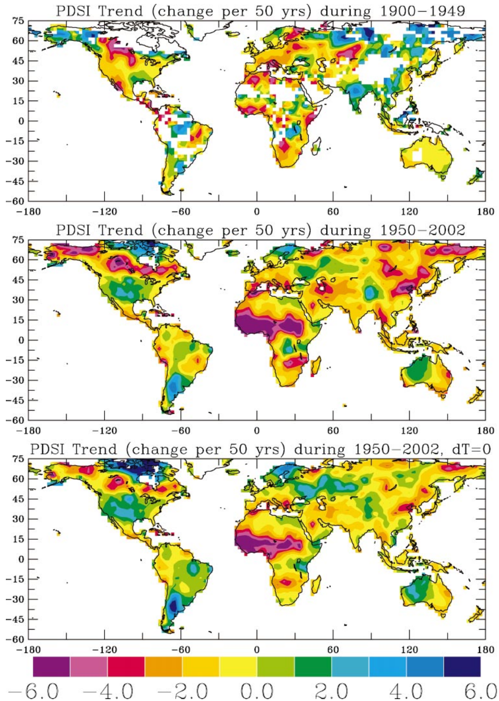
FIG. 7. Maps of linear trends of PDSI [change (50 yr) -1 , calculated with both precipitation and temperature changes] during (top) 1900–49 and (middle) 1950–2002. (bottom) The trends of PDSI calculated without temperature changes. Red (blue) areas indicate drying (wetting).
